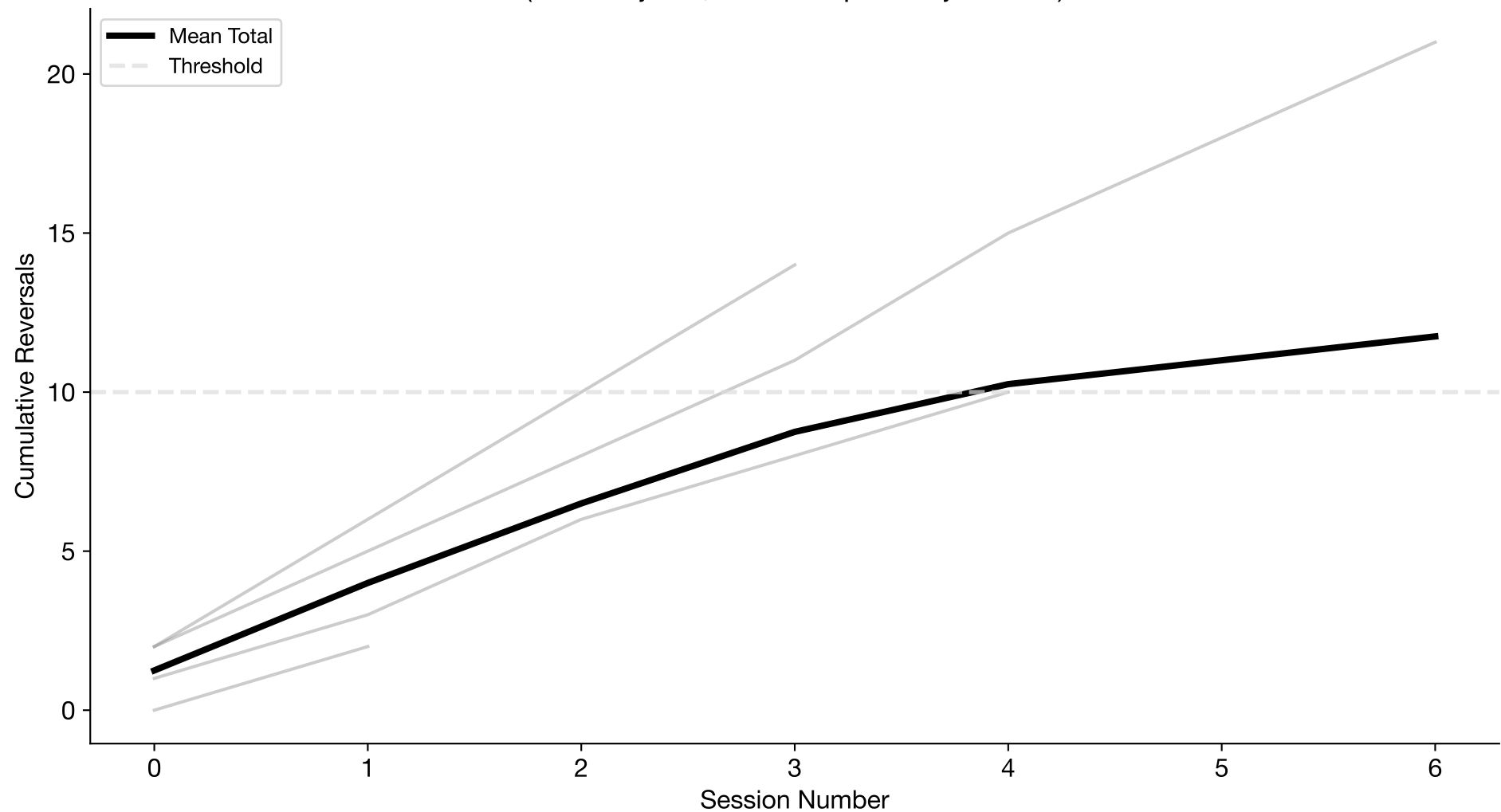
Cumulative Total Reversals Over Time (n=4 subjects; sessions per subject=2-7)
